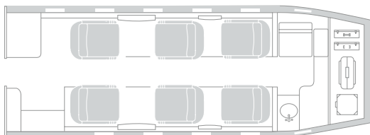
VIP Layout Setup
